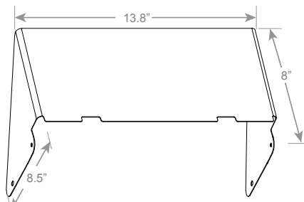
Glare Shield for PMPALDSR-403530L-3CCT PMPALDSR-403530L-3CCT-GS
