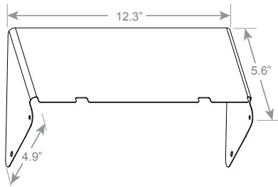
Glare Shield for PMPALDSR-242115L-3CCT PMPALDSR-242115L-3CCT-GS
