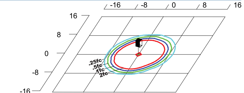
PBOGRLQF1X15U5K Type V Grid in feet, Mounting Height = 3.5 ft.
