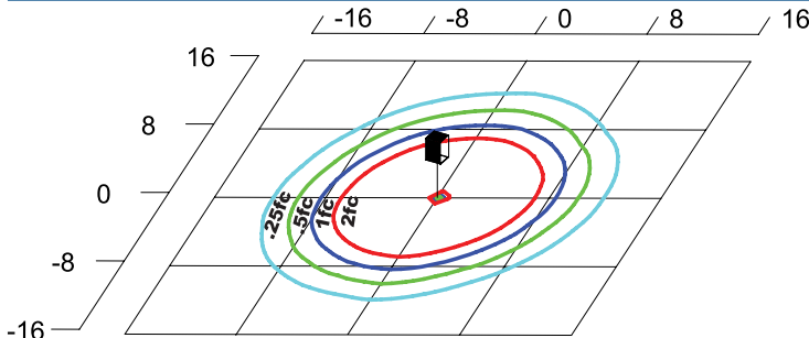
PBOGQF1X15U5K Type V Grid in feet, Mounting Height = 3.5 ft.
