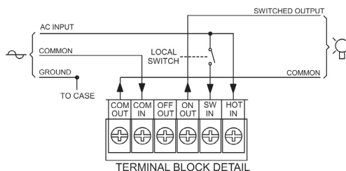
Diagram 4. SWITCHED LOADS
