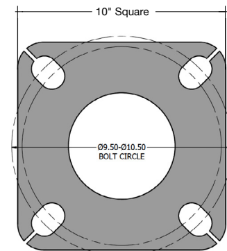
8" X 8" X .75" THICK BASE PLATE
