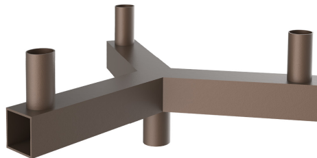
Part #: PTN-BH-SQ-180-3Y Tenon: Square Bullhorn 3-Head Y-Adapter Bracket EPA: 1.9
