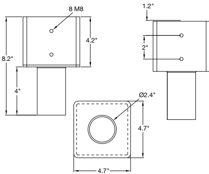
Part #: PTN-SQ-4 Tenon: Square 4" Pole Reducer to 2.36" Bracket EPA: 0.3
