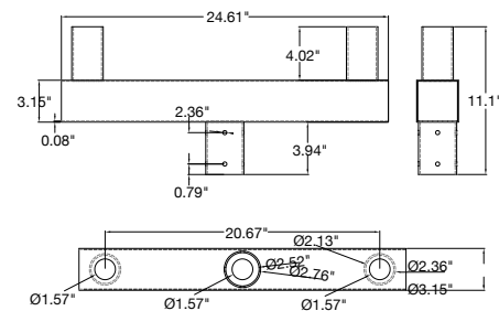
Part #: PTN-BH-SQ-180-2S Tenon: Square Bullhorn 2-Head Adapter Bracket EPA: 1.2
