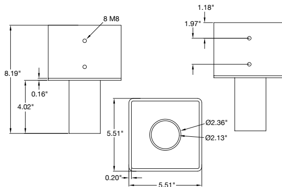
Part #: PTN-SQ-5 Tenon: Square 5" Pole Reducer to 2.36" Bracket EPA: 0.35
