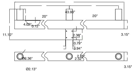
Part #: PTN-BH-SQ-180-3S Tenon: Square Bullhorn 3-Head Adapter Bracket EPA: 1.9
