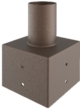
Part #: PTN-SQ-4 Tenon: Square 4" Pole Reducer to 2.36" Bracket EPA: 0.3
