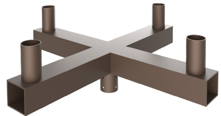
Part #: PTN-BH-SQ-90-4X Tenon: Square Bullhorn 4-Head X-Adapter Bracket EPA: 2
